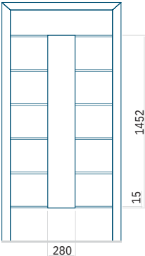
Technical drawing
