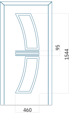
Technical drawing
